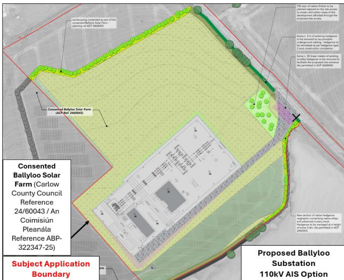
Figure 02: Proposed 110kV AIS Substation Option
