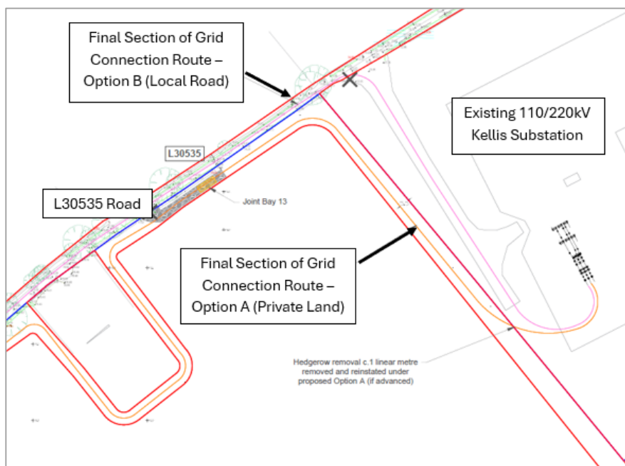
Figure 05: Final Underground Cabling Options on Public Road / Private Lands
