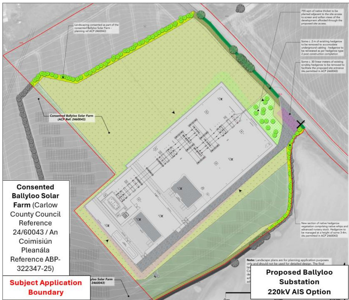
Figure 03: Proposed 220kV AIS Substation Option
